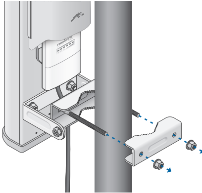
Lower Bracket Connection Overview
