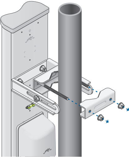
Upper Bracket Connection Overview
